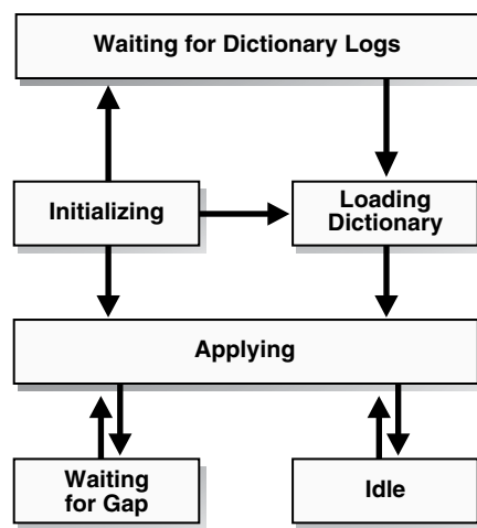
Figure 10-2 Progress States During SQL Apply Processing
